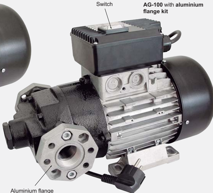
Aluminium flange
